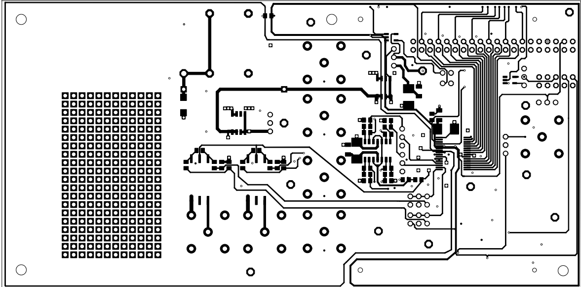
Figure 3–3. Printed-Circuit Board Layer 1
