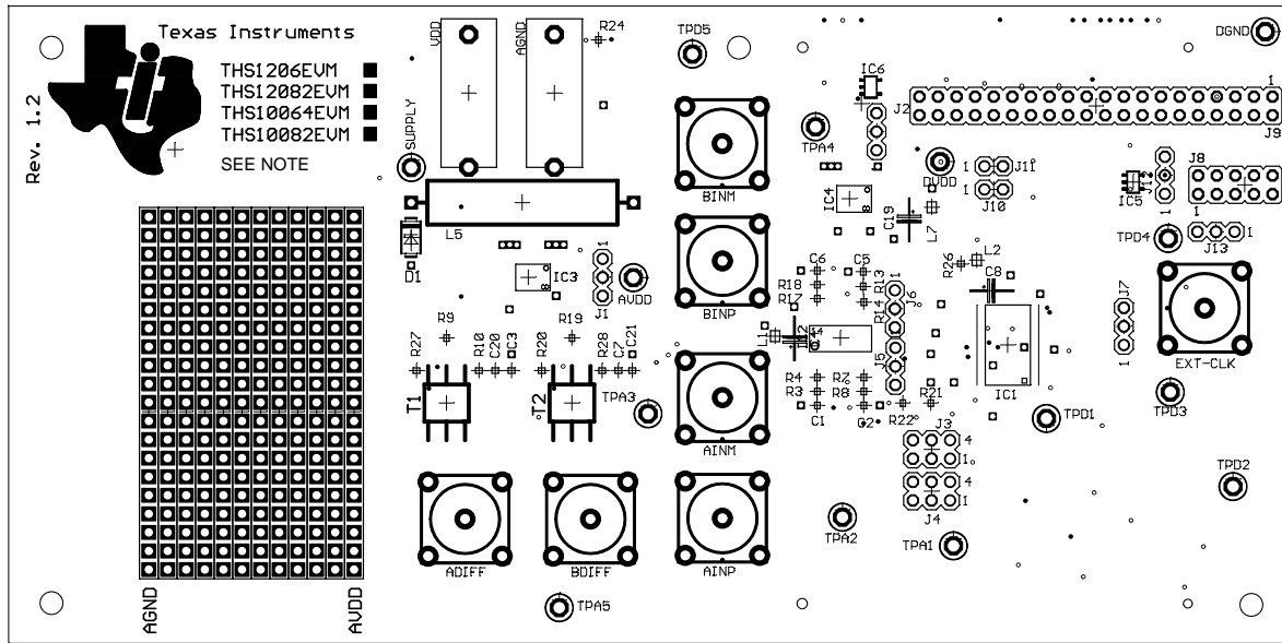
Figure 3–1. Silkscreen (Top)
