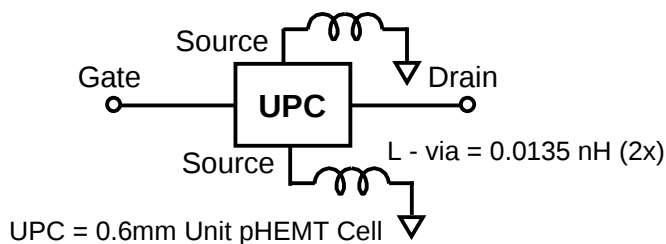
Unit pHEMT cell Reference Plane
