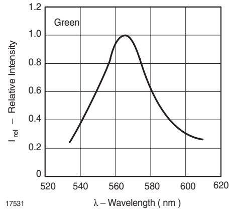
17531 Figure 18. Relative Intensity vs. Wavelength
