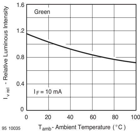
95 10035 Figure 15. Rel. Luminous Intensity vs. Ambient Temperature
