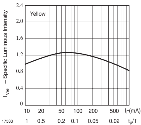
17533 Figure 11. Specific Luminous Intensity vs. Forward Current
