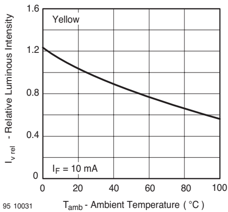
95 10031 Figure 10. Rel. Luminous Intensity vs. Ambient Temperature
