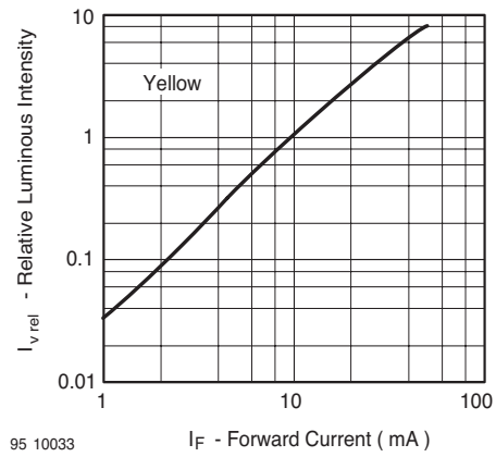
95 10033 Figure 12. Relative Luminous Intensity vs. Forward Current
