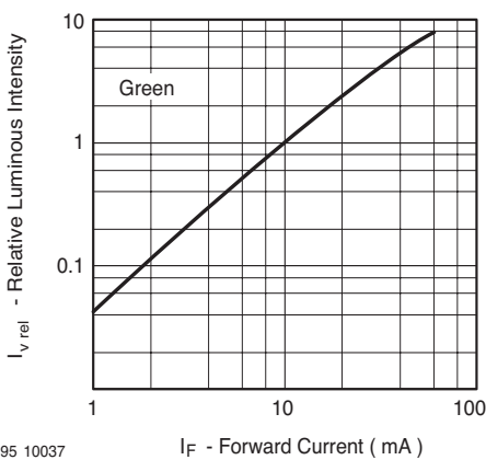
95 10037 Figure 17. Relative Luminous Intensity vs. Forward Current
