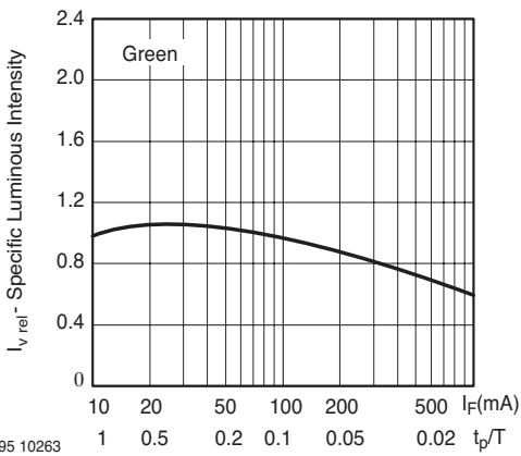
95 10263 Figure 16. Specific Luminous Intensity vs. Forward Current
