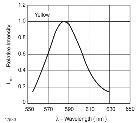
17530 Figure 13. Relative Intensity vs. Wavelength
