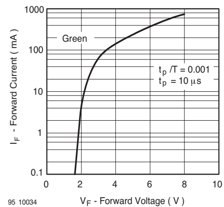
95 10034 Figure 14. Forward Current vs. Forward Voltage
