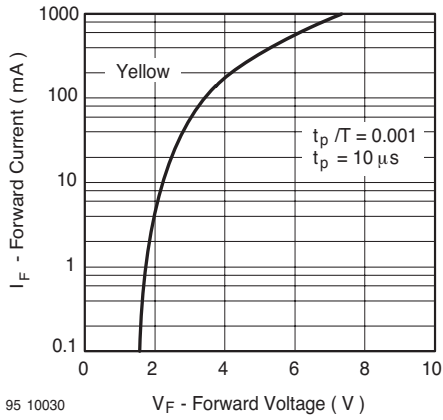
95 10030 Figure 9. Forward Current vs. Forward Voltage
