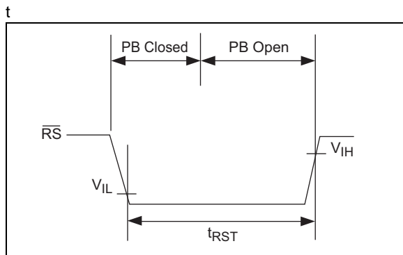
FIGURE 3-2: RS Pulled Low By Push-Button Reset
