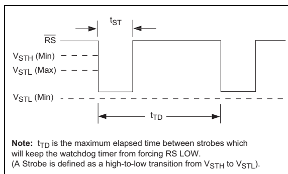
FIGURE 3-1: Watchdog Strobe
