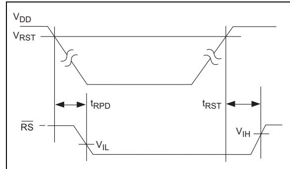
FIGURE 3-3: Power-Up/Down Reset Timing
