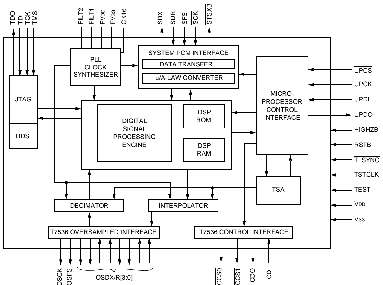
Figure 4. T7531A Block Diagram
