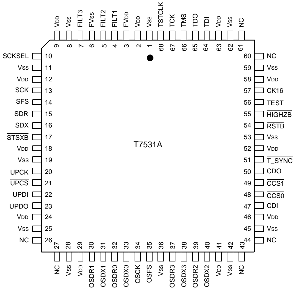
Figure 8. T7531A 68-Pin PLCC
