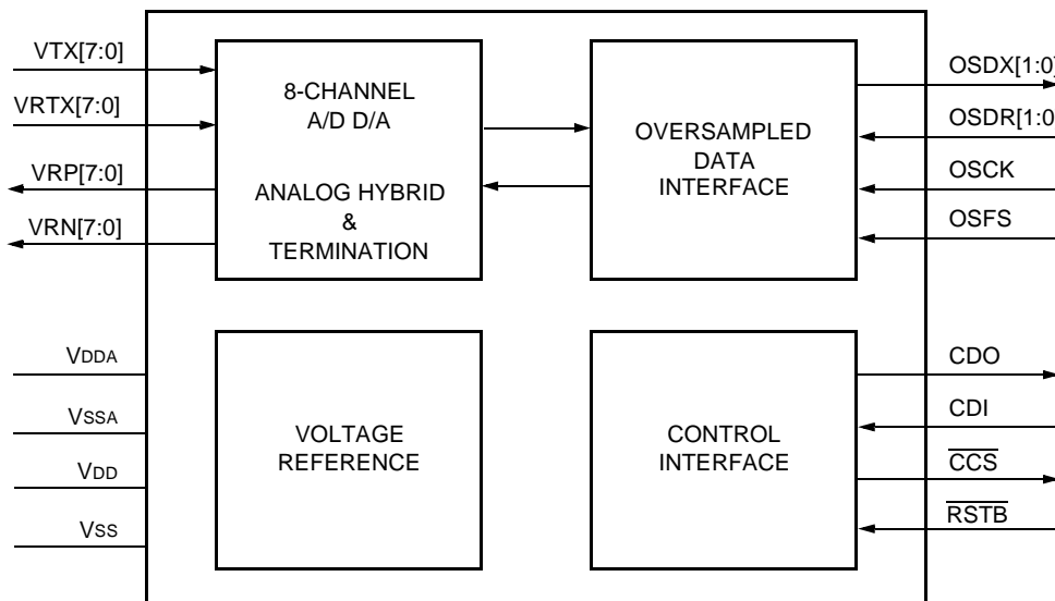
Figure 2. Block Diagram of T7536 Octal Converter
