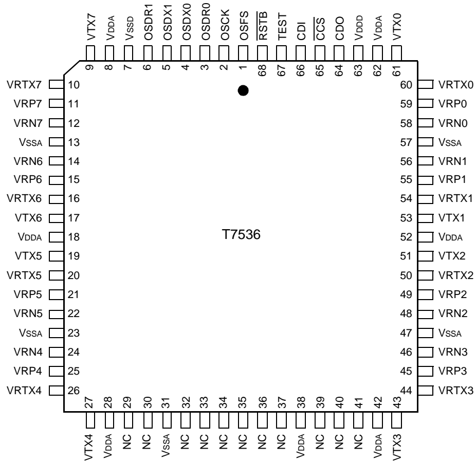
Figure 7. T7536 68-Pin PLCC
