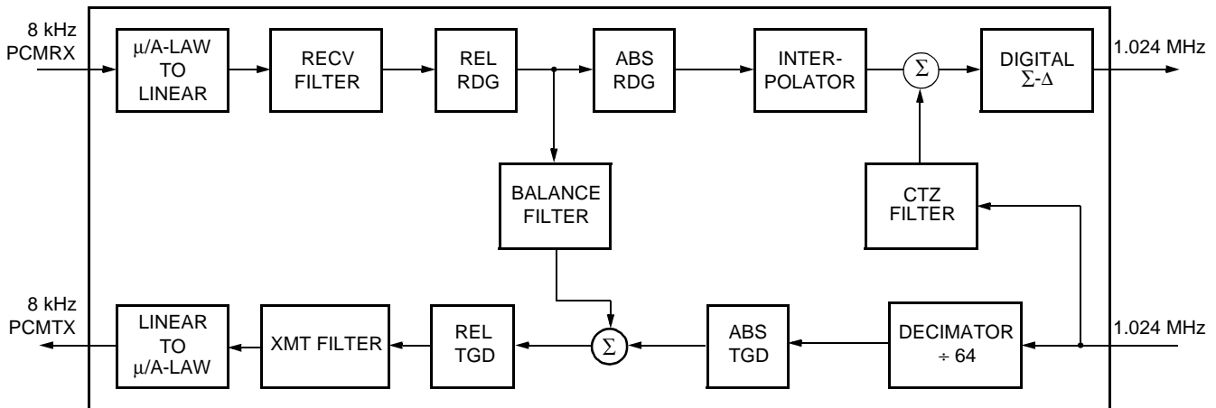
Figure 5. T7531A Digital ac Path
