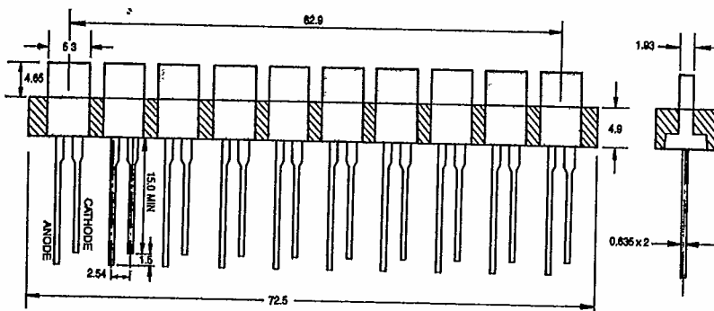
H-3 1.8x5.3m/m ARRAY SOCKET 10 SEQUENT
