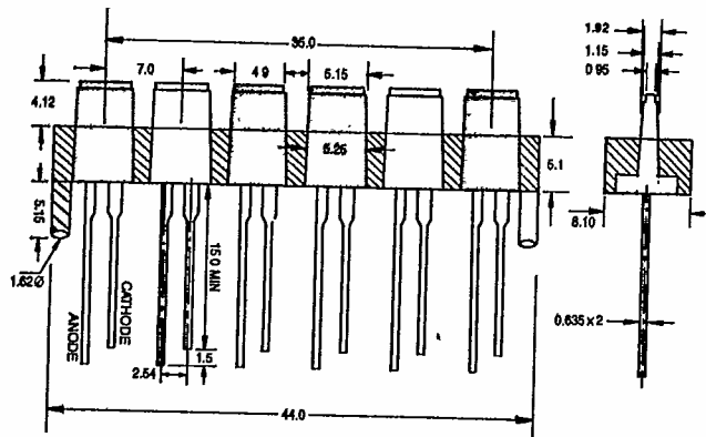
H-1 1x5m/m ARRAY SOCKET 6 SEQUENT
