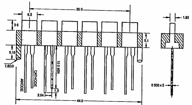
H-4 1.8x5.3m/mARRAY SOCKET 6 SEQUENT
