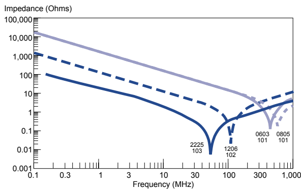
FIGURE 4. Impedance versus Frequency C0G Dielectric
