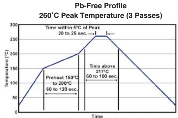
Time/Temperature Soldering Profile
