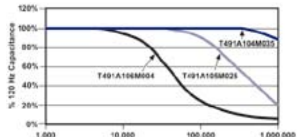
FIGURE 1 Typical Effect of Frequency upon Capacitance
