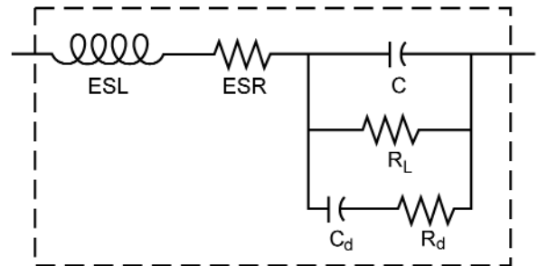
Figure 5. The Real Capacitor
