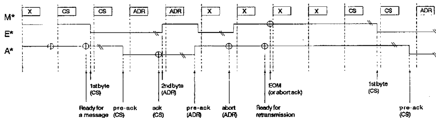
TWO BYTES MESSAGE ABORTED ON THE SECOND AND RETRANSMITTED
