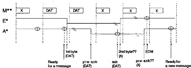
ONE BYTE MESSAGE - NORMAL TRANSMISSION
