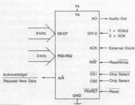
Signal Diagram
