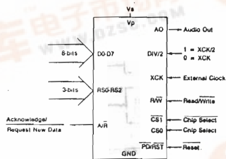
Signal Diagram
