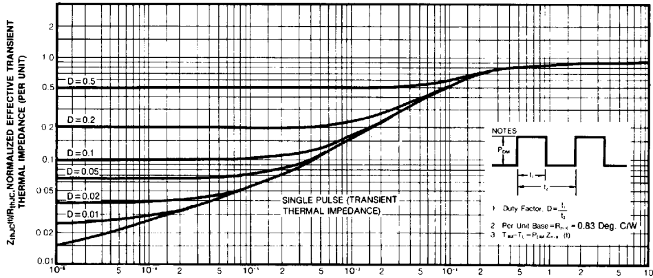
(1. SQUARE WAVE PULSE DURATION (SECONDS)) Maximum Effective Transient Thermal Impedance Junction-to-Case Vs. Pulse Duration
