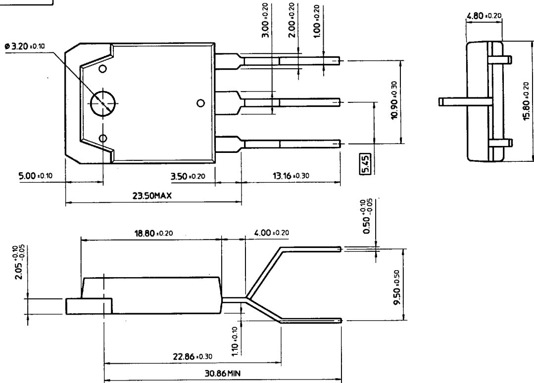
TO-3P (2)
