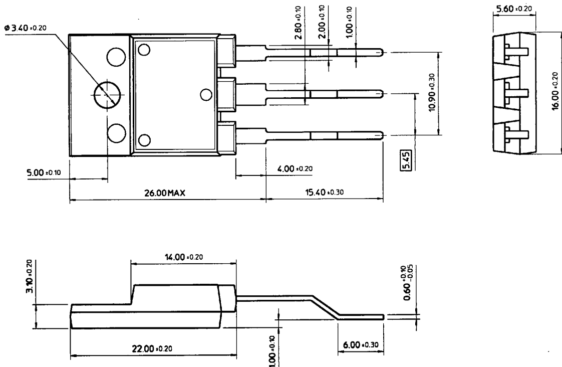
TO-3PF (1)
