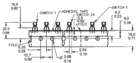
TAPE STYLE T2
