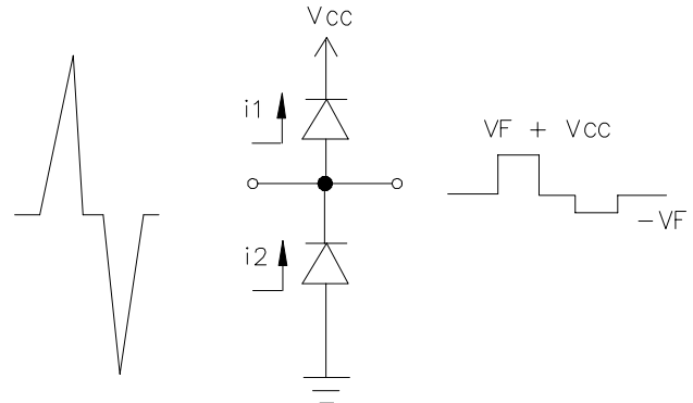
Figure 3 - "Rail-To-Rail" Protection Topology (First Approximation)
