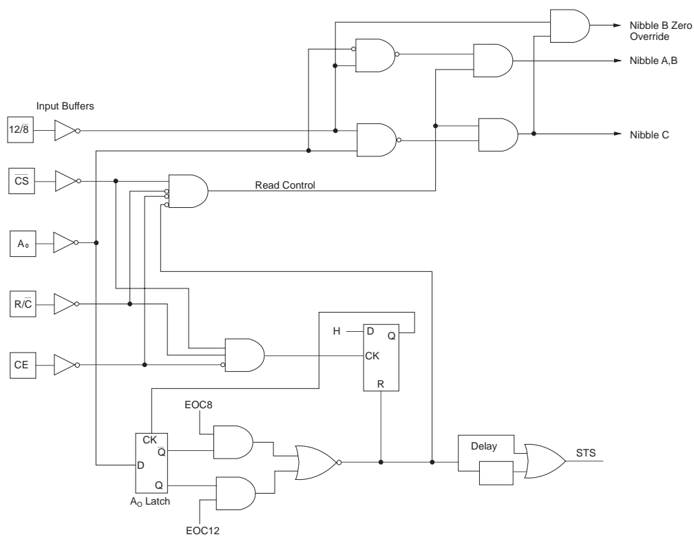
Figure 10 - Control Logic
