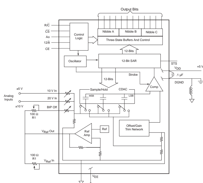
Figure 6 - Bipolar Input Connections
