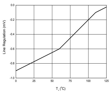
Figure 6. Line Regulation vs. Temperature
