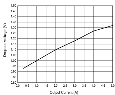
Figure 4. Dropout Voltage vs. Output Current
