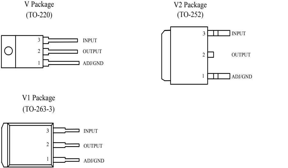
Figure 2. Pin Configuration of SP1084 (Top View)
