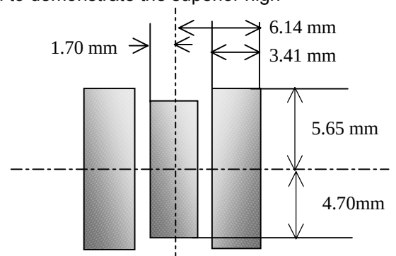
Solder Pad Layout
