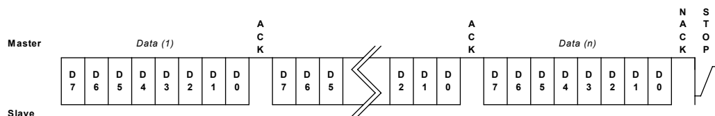
Figure 12 - Configuration Register Read
