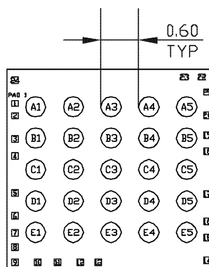
BOTTOM VIEW
