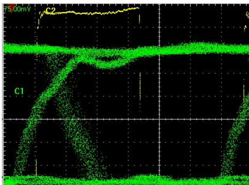
Figure 12. Eye Diagram
