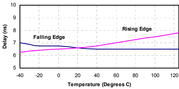
Figure 9. Propagation Delay vs. Temperature 3.3 V Operation
