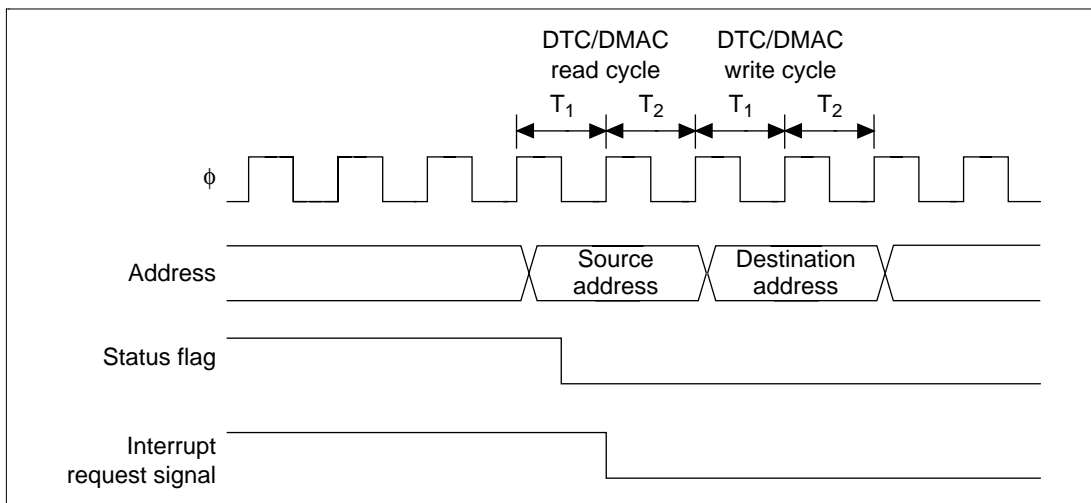
Figure 12.75 Timing of Status Flag Clearing by DTC/DMAC Activation
