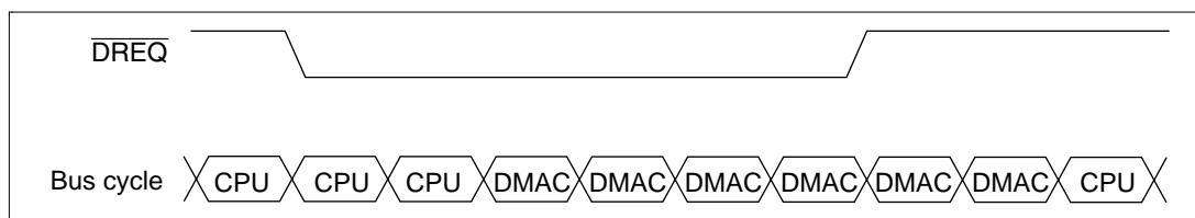
Figure 11.13 DMA Transfer Example in the Burst Mode
