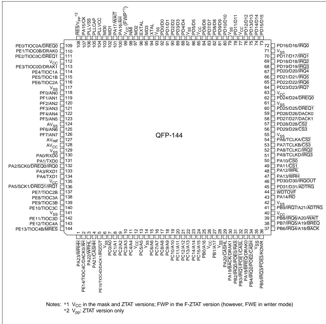
Figure 1.5 shows the pin arrangement for the QFP-144 (top view).
