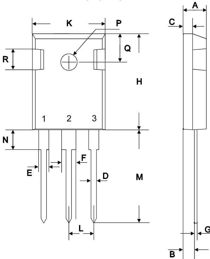
PG-TO247-3-1
