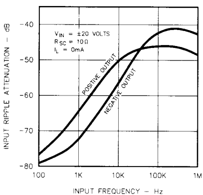
FIGURE 11. RIPPLE REJECTION
