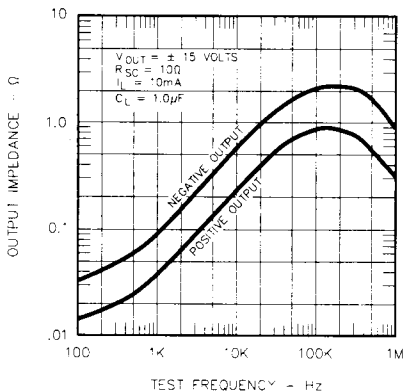
FIGURE 12. OUTPUT IMPEDANCE
