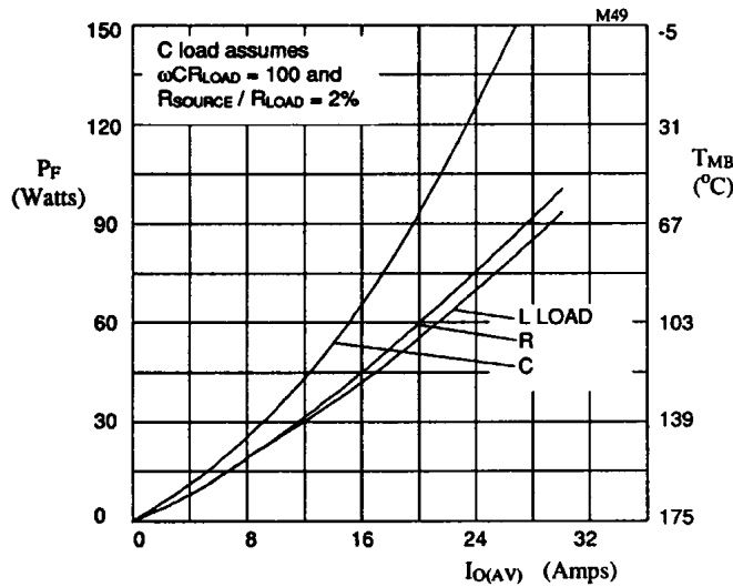
Figure 6. Forward power dissipation and maximum allowable mounting base temperature as a function of output current for sinusoidal operation, for SET061203 and SET061212.
