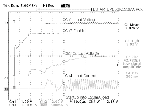
Start-Up Conditions for 4.0V Output
