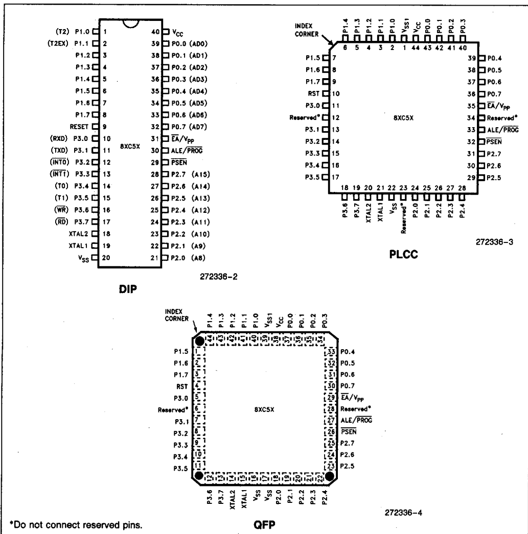
Figure 2. Pin Connections
