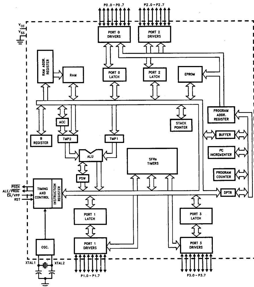
Figure 1. 8XC5X Block Diagram
