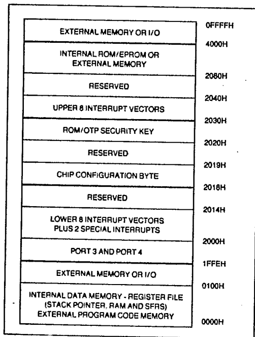
Figure 2. Memory Map
