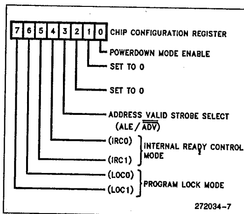
Figure 3. Chip Configuration (2018H)
