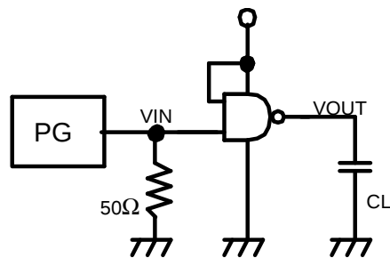
Measurement Circuit
