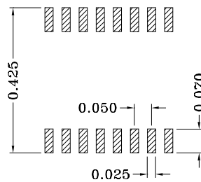
SUGGESTED PCB PAD LAYOUT
