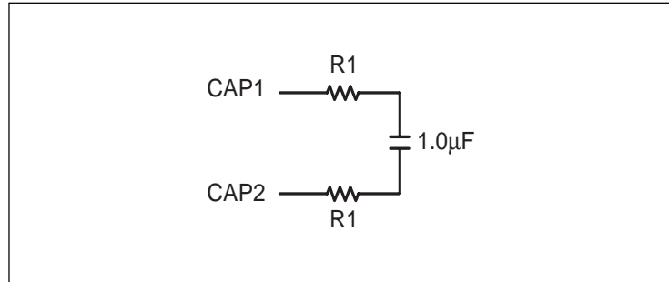
Figure 7. External Loop Filter
