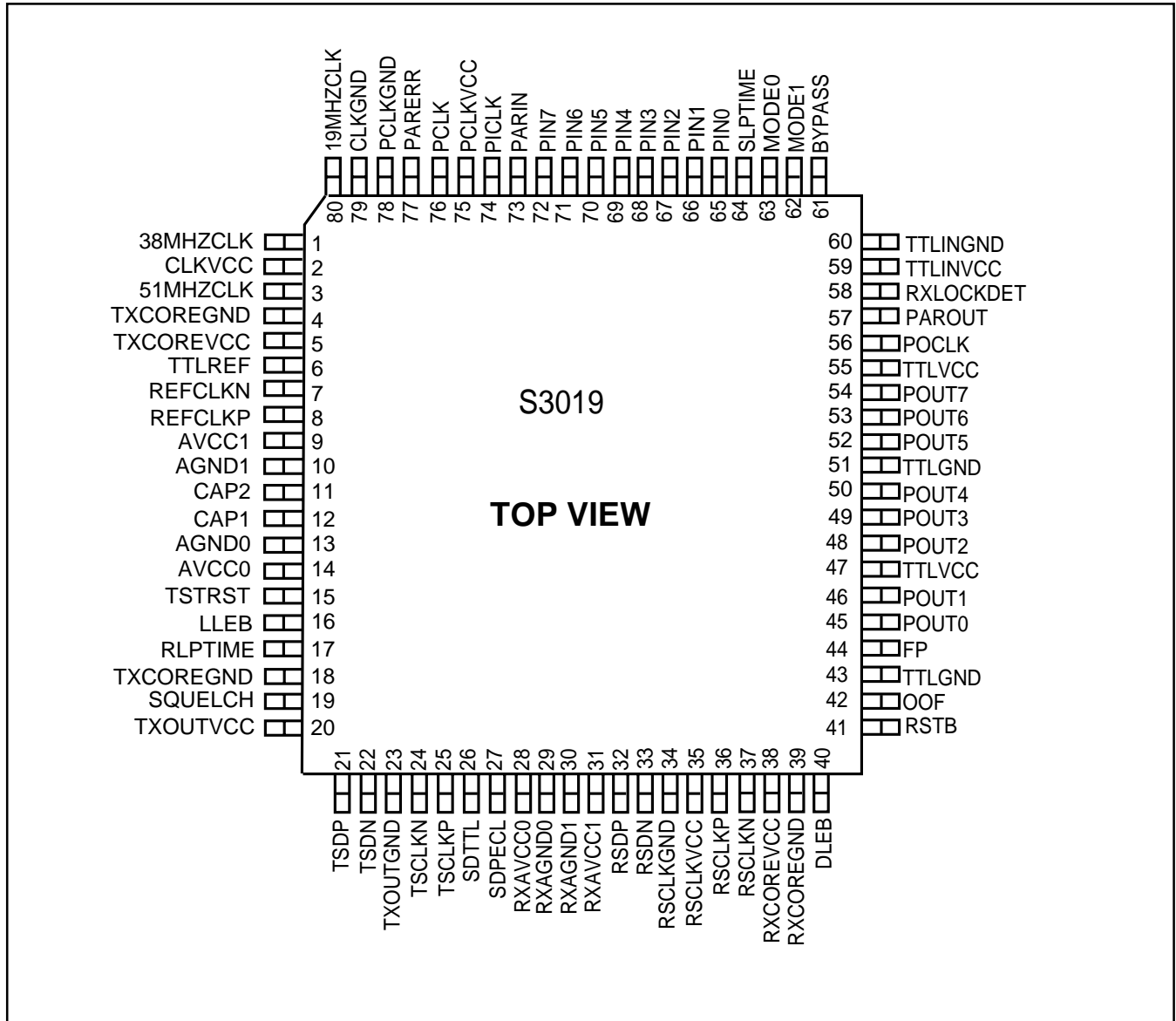
Figure 7. Pinout Assignments
