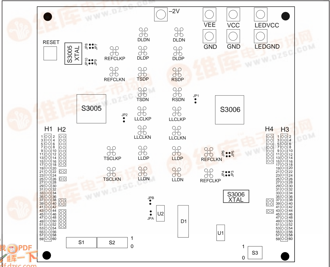
Figure 1. Board Layout
