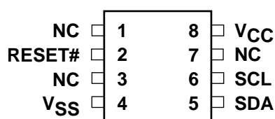
SMS24163 8-Pin PDIP or 8-Pin SOIC
