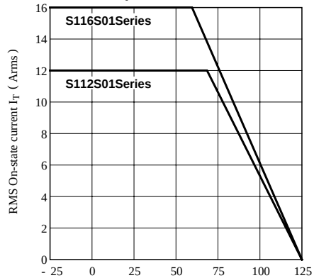
Fig. 3 RMS ON-state Current vs. Case Temperature
