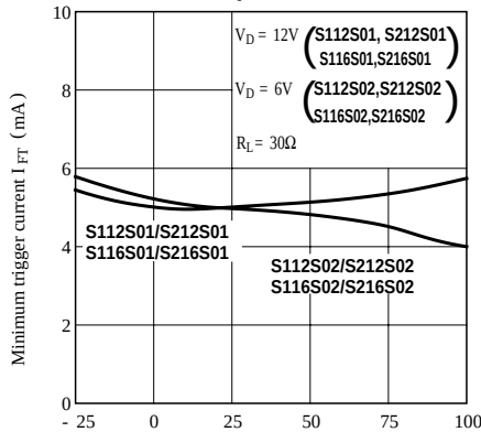
Fig. 9 Minimum Trigger Current vs. Ambient Temperature
