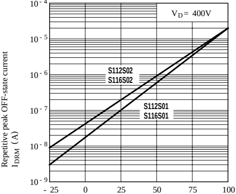
Fig.10 Repetitive Peak OFF-state Current vs. Ambient Temperature (S112S01/ S112S02/ S116S01/ S116S02)
