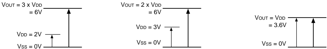
Triple step-up potential relationship Double step-up potential relationship VOUT = VDD potential relationship
