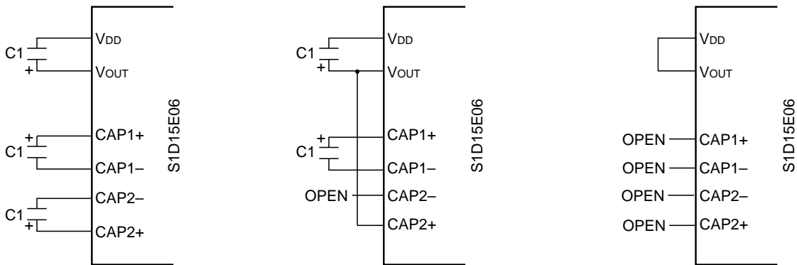
① Triple, double step-up or VOUT = VDD
