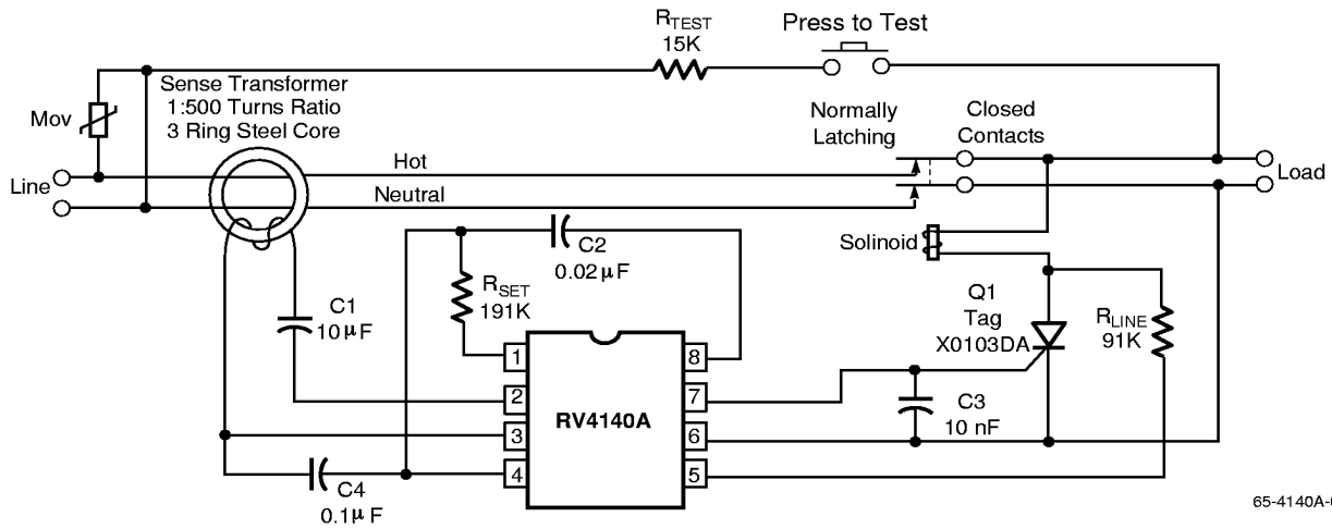
Figure 1. Appliance Leakage Detector Circuit Application
