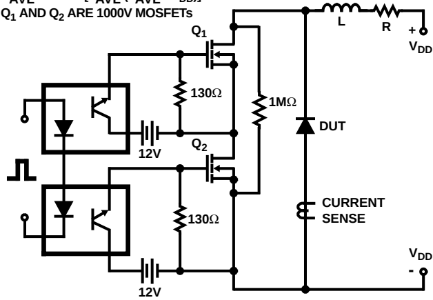
FIGURE 9. AVALANCHE ENERGY TEST CIRCUIT
