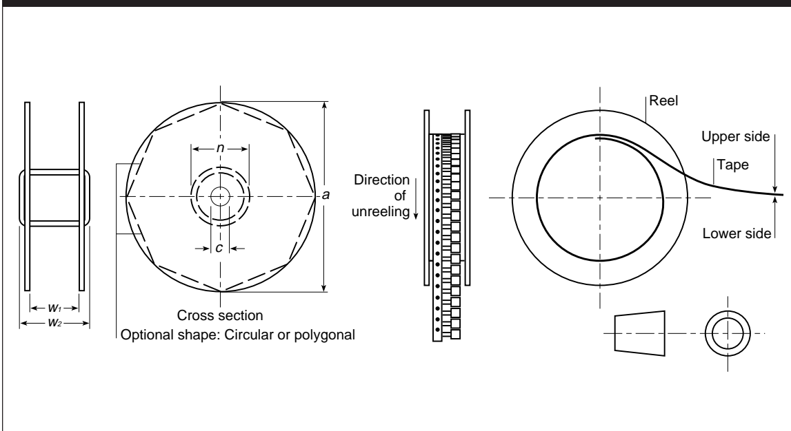
Figure 2: Reel Dimensions
