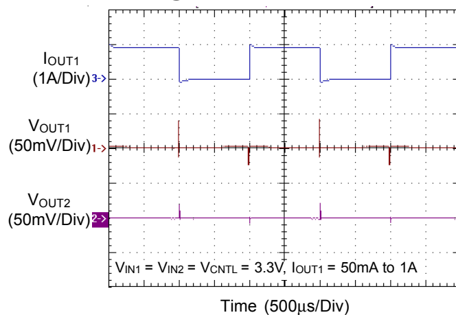
V_{OUT1} @ 1A Load Transient Response
