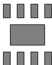
Figure 5 (b). Copper Area = 10\text{mm}^2 , \theta_{JA} = 64^{\circ}\text{C/W}
