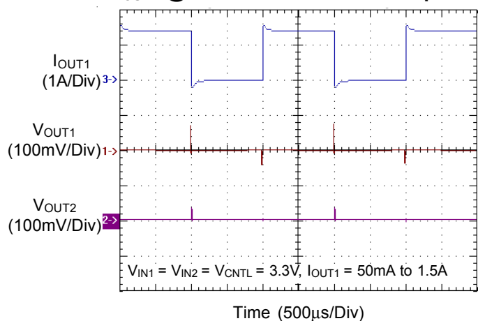
V_{OUT1} @ 1.5A Load Transient Response
