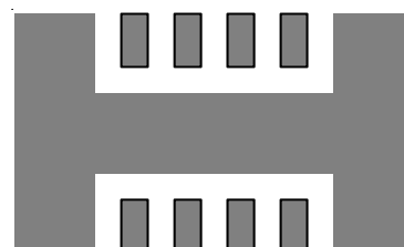
Figure 5 (d). Copper Area = 50\text{mm}^2 , \theta_{JA} = 51^{\circ}\text{C/W}
