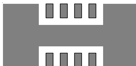
Figure 5 (e). Copper Area = 70\text{mm}^2 , \theta_{JA} = 49^{\circ}\text{C/W}
