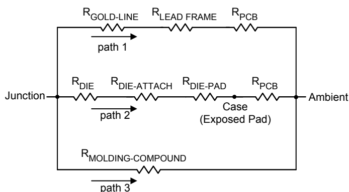
Figure 2. Thermal Resistance Equivalent Circuit
