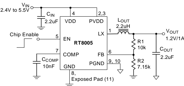
Recommended component selection for Typical Application Circuit.
