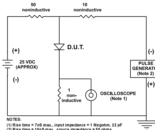
FIGURE 5. REVERSE RECOVERY TEST SETUP AND TIME CHARACTERISTIC
