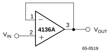
Figure 23. Voltage Follower
