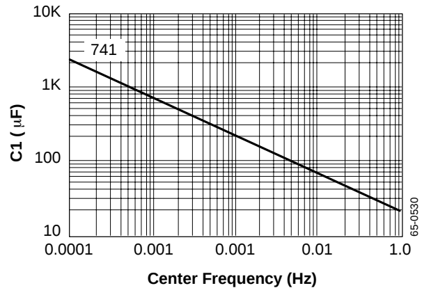
Figure 33. Notch Frequency vs. C1
