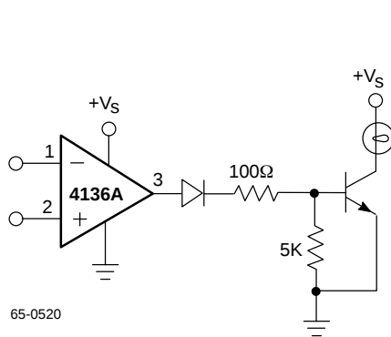
Figure 21. Lamp Driver
