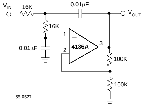
Figure 25. DC Coupled 1kHz Lowpass Active Filter
