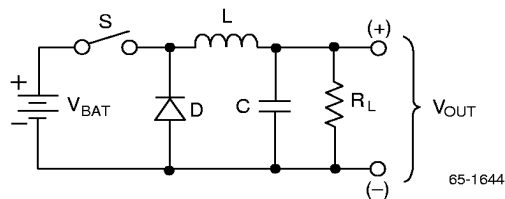
Figure 10. Simple Step-Down Converter
