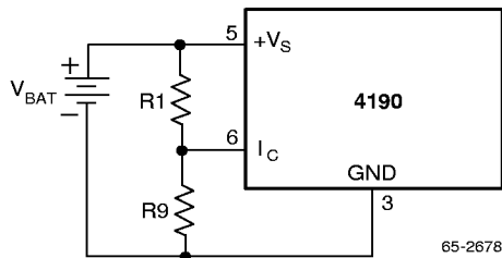
Figure 14. Automatic Shutdown
