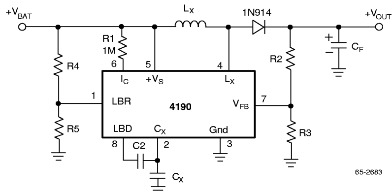
Figure 19. Step-Up Voltage Dependent Oscillator
