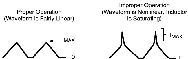
Figure 28. Inductor Current Waveforms
