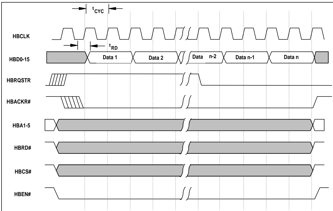
Figure 4-5. Host DMA Demand Mode Read, DMAMODE = 1
