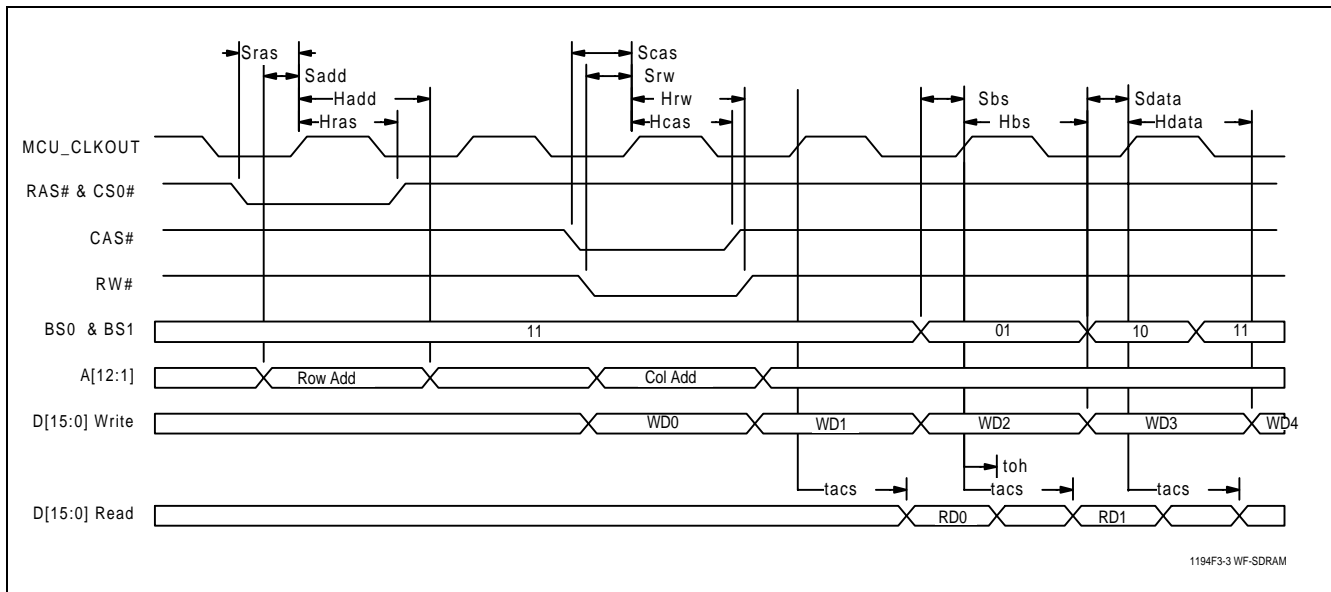
Figure 3-7. SDRAM Interface Timing
