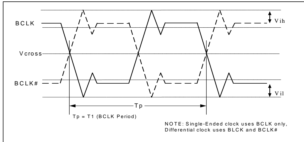
Figure 9. Clock Waveform
