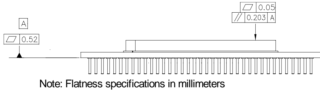
Figure 23. FC-PGA2 IHS Flatness Specification
