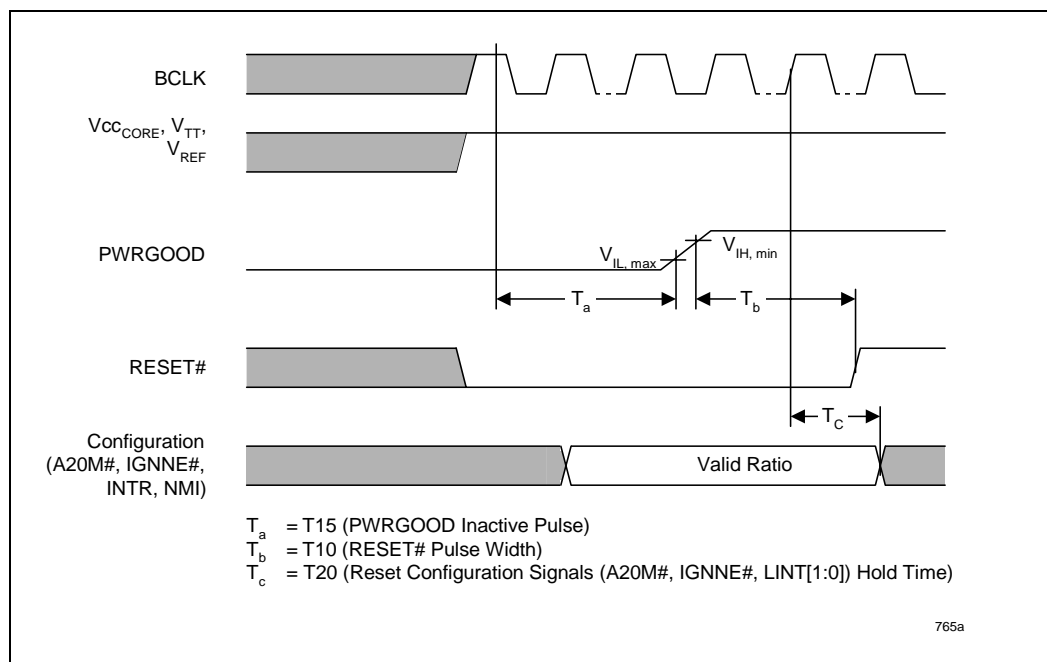
Figure 15. Power-On Reset and Configuration Timings
