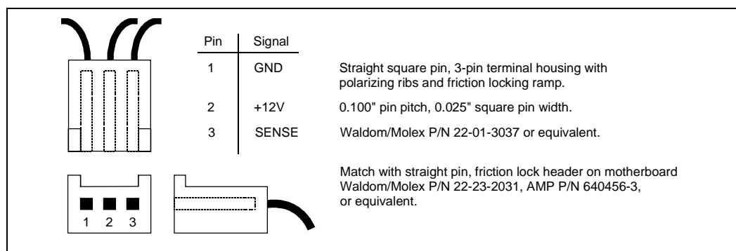
Figure 33. Boxed Processor Fan Heatsink Power Cable Connector Description
