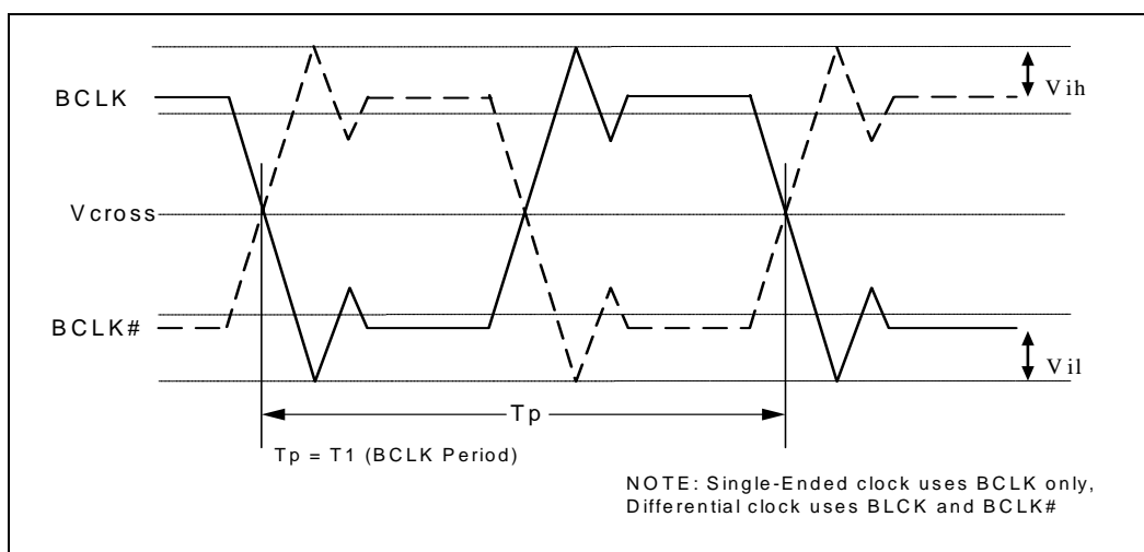
Figure 9. Clock Waveform
