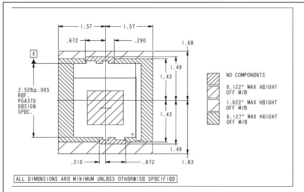
Figure 24. Component Keep-Out
