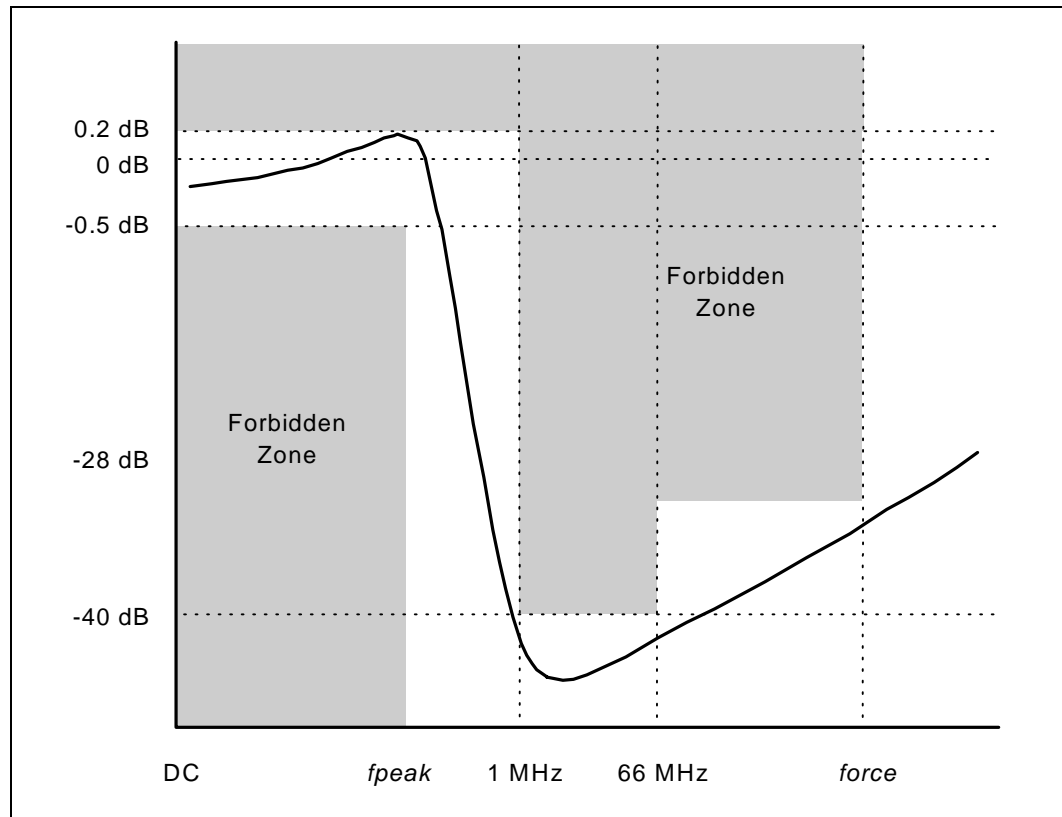
Figure 4. PLL Filter Specification
