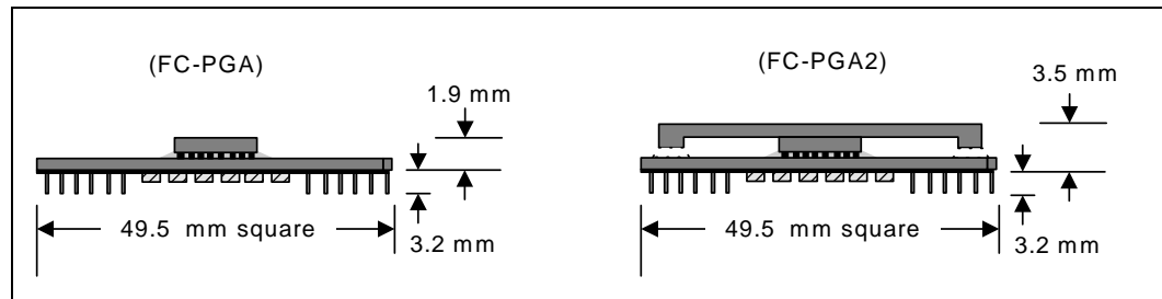
Figure 28. Comparison between FC-PGA and FC-PGA2 package
